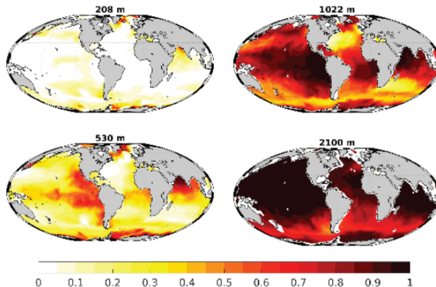
Figure 5.3 Maps of the fraction of CO 2 retained after 100 years for injection depths of 208, 530, 1,022, and 2,100 meters in the purposeful sequestration metrics modeling of Siegel et al. (2021b).
